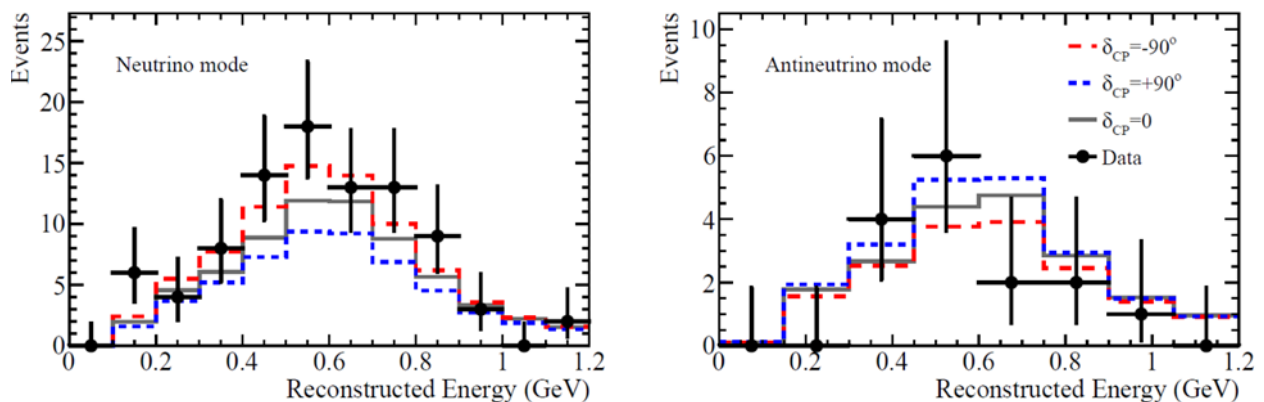
Fig.3 The observed electron neutrino (left) and electron antineutrino (right) candidate events with predictions for maximal neutrino enhancement (red, long dash) and maximum antineutrino enhancement (blue, short dash).
